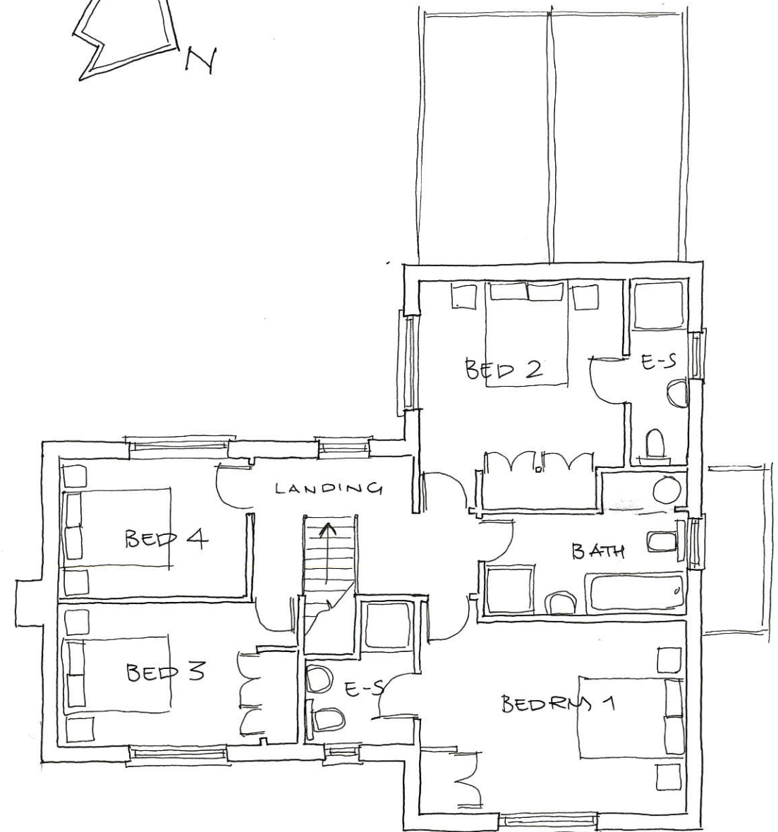
FIRST FLOOR ~ 1:100
