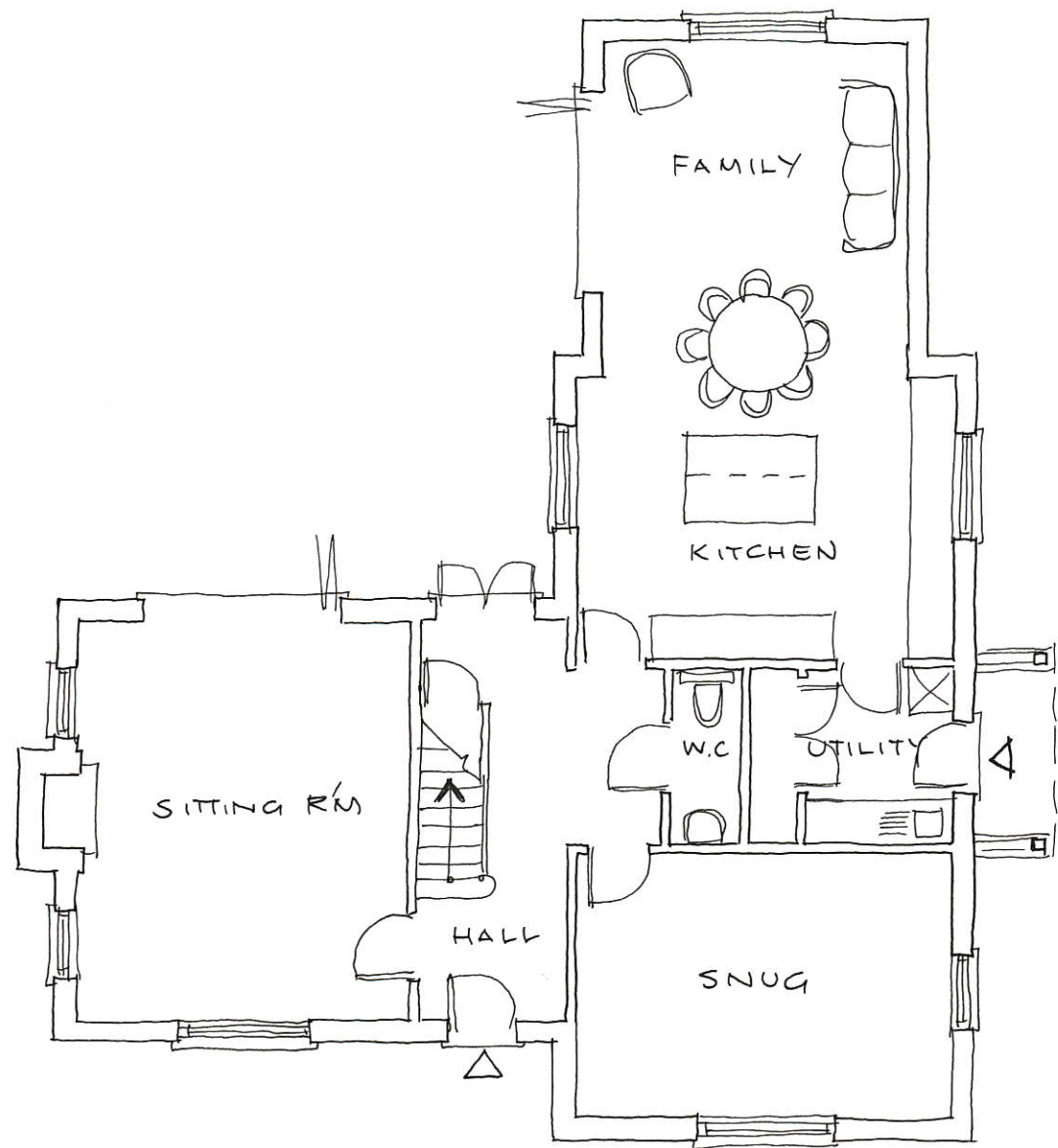
GROUND FLOOR - PLOT 1
