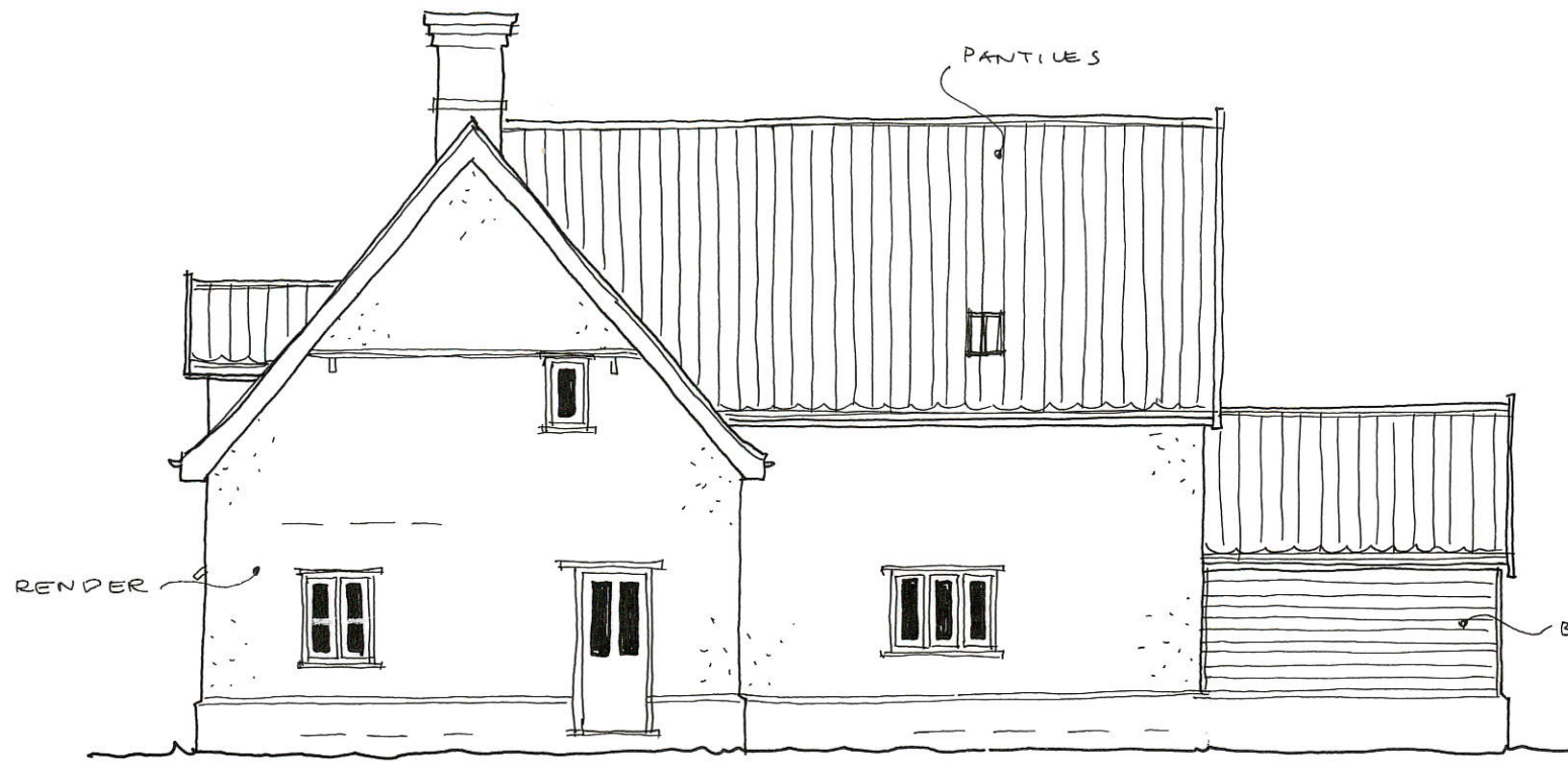
NORTH ELEVATION ~
