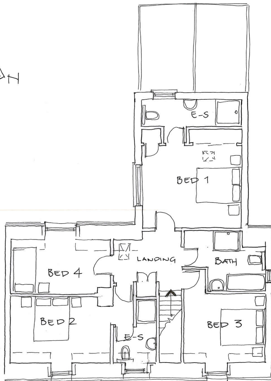
FIRST FLOOR ~ 1:100
